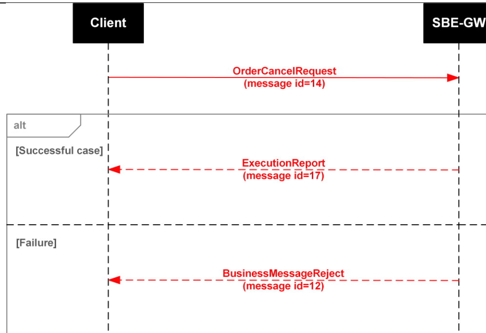
Figure 13. Diagram. Client order cancellation (by client)
